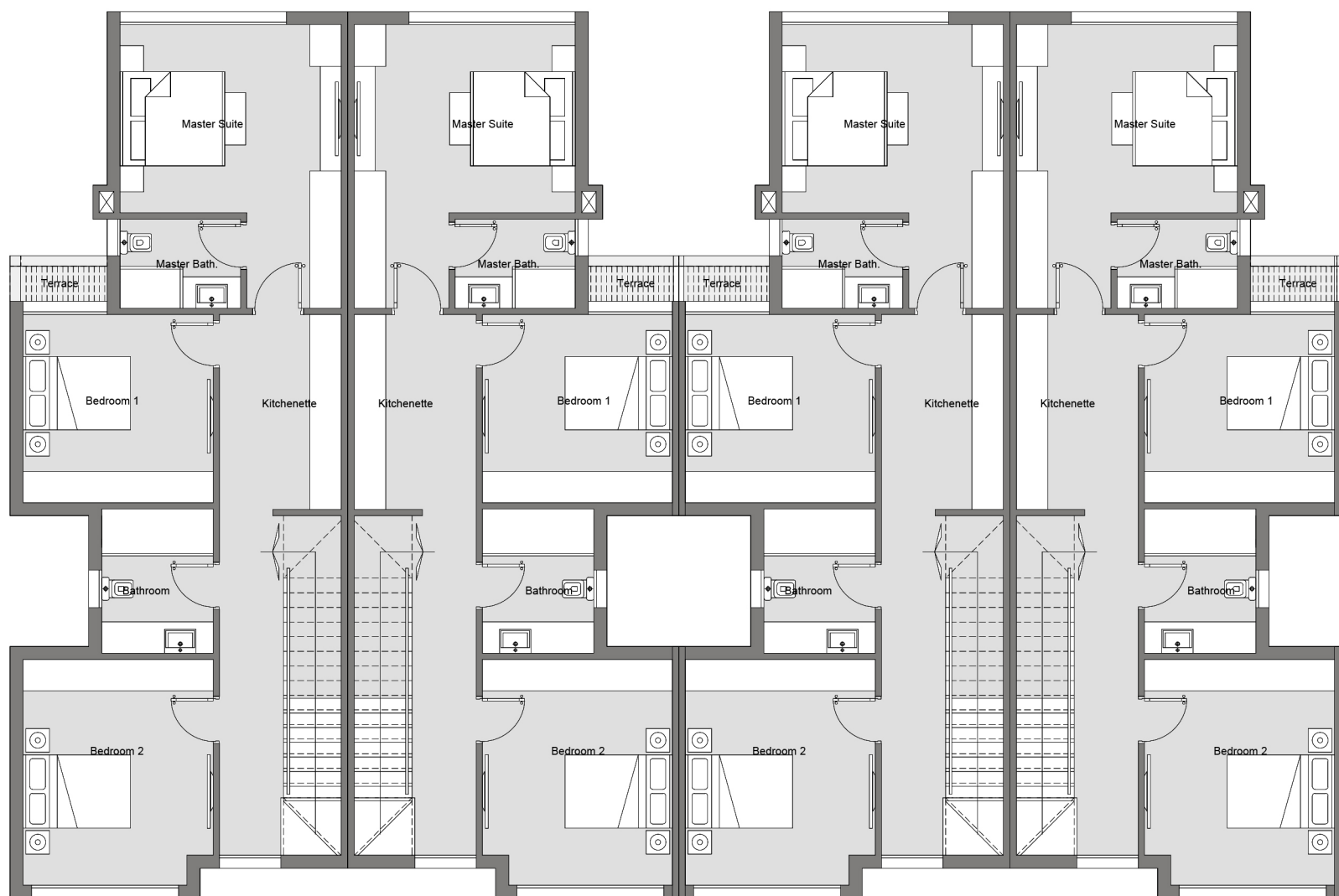
First Floor
